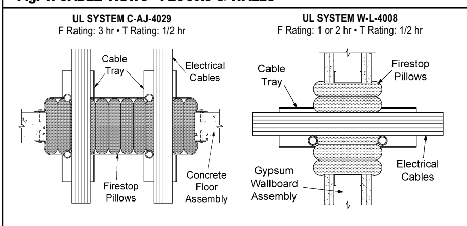
Fig. 1: CABLE TRAYS - FLOORS & WALLS
